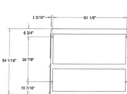
10 TON AIR HANDLER (DUAL CIRCUIT) DIMENSIONAL DRAWING
