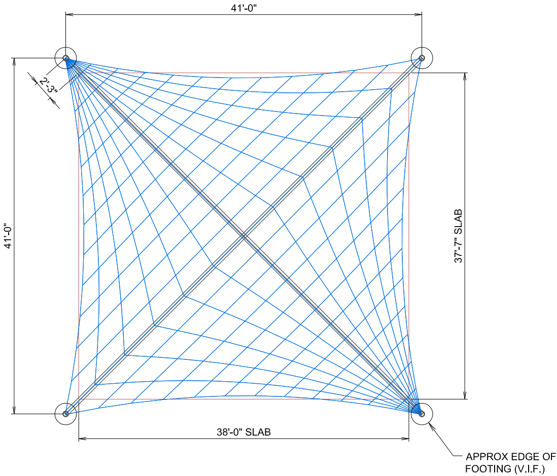
PLAN VIEW
