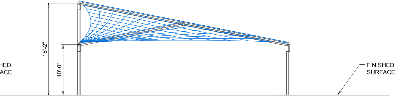
WEST ELEVATION
